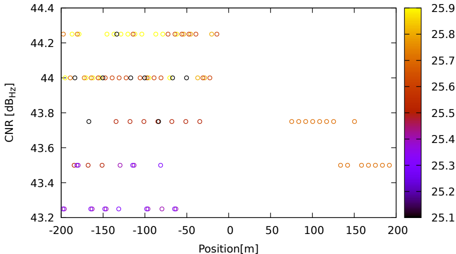
CNR vs position for C16 (B2) on LeicaGS18 - DOY 262 jam. 2
