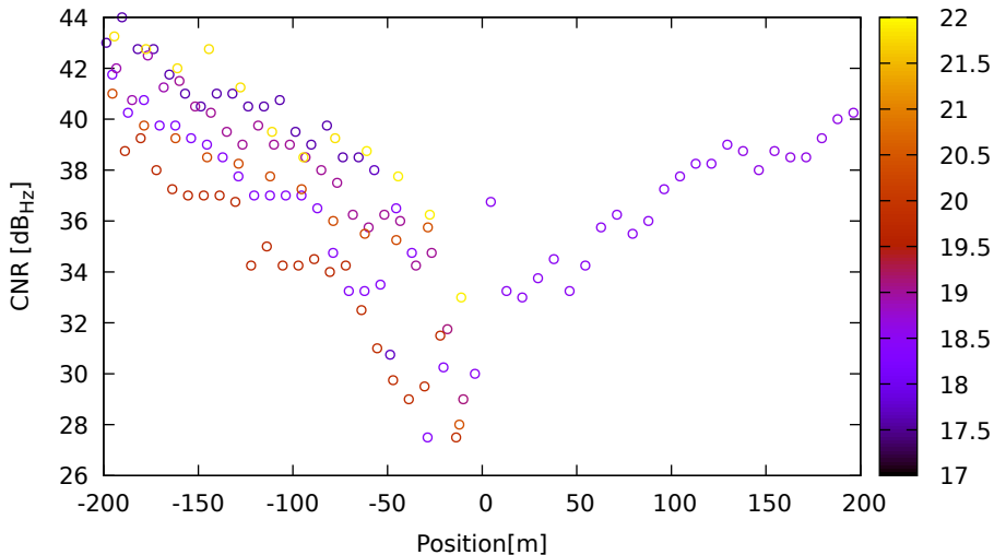
CNR vs position for C27 (B1) on LeicaGS18 - DOY 262 jam. 1
