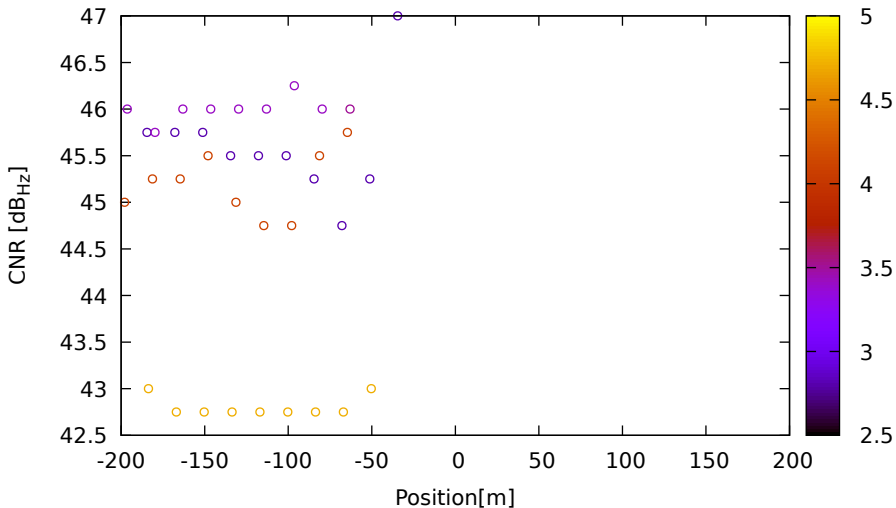
CNR vs position for E03 (E5a) on LeicaGS18 - DOY 262 jam. 2
