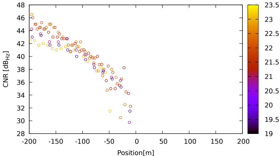
CNR vs position for E04 (E1) on LeicaGS18 - DOY 262 jam. 1
