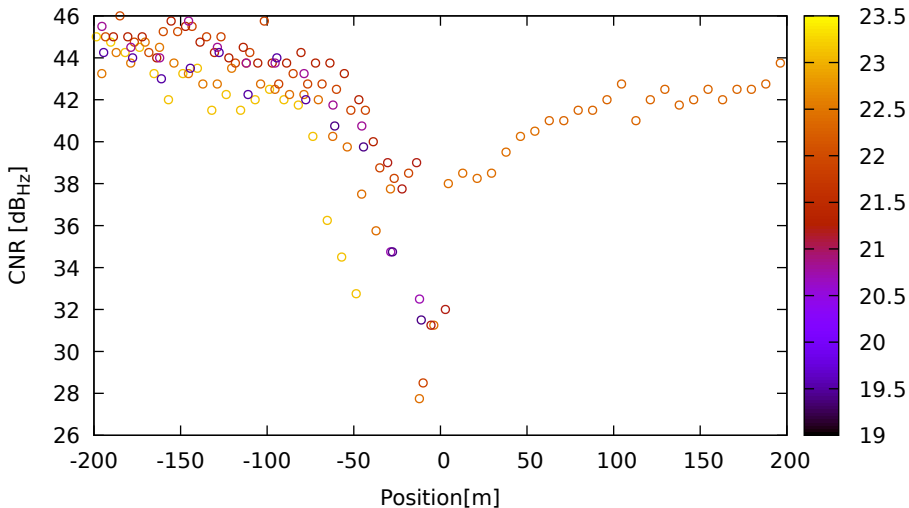
CNR vs position for E04 (E5a) on LeicaGS18 - DOY 262 jam. 1
