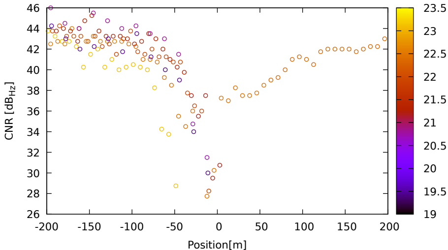
CNR vs position for E04 (E5b) on LeicaGS18 - DOY 262 jam. 1
