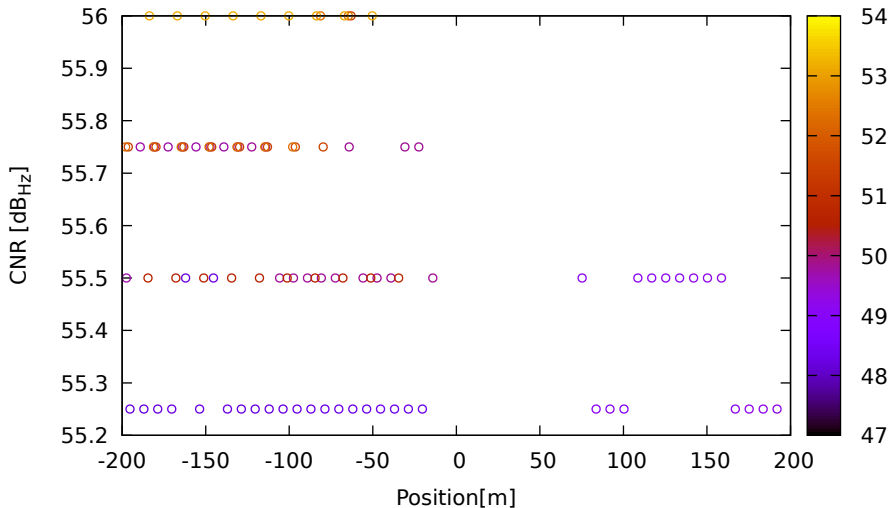
CNR vs position for E05 (E5) on LeicaGS18 - DOY 262 jam. 2
