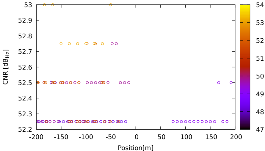
CNR vs position for E05 (E5a) on LeicaGS18 - DOY 262 jam. 2
