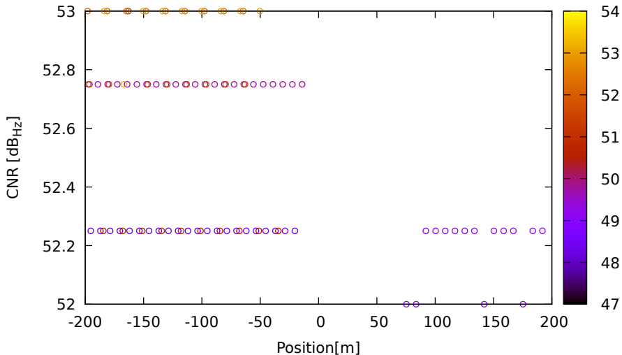
CNR vs position for E05 (E5b) on LeicaGS18 - DOY 262 jam. 2
