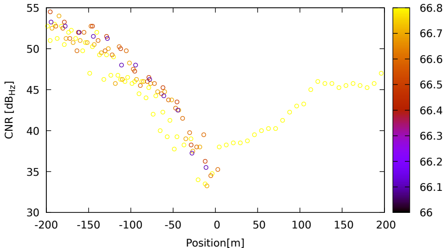
CNR vs position for E09 (E5) on LeicaGS18 - DOY 262 jam. 1
