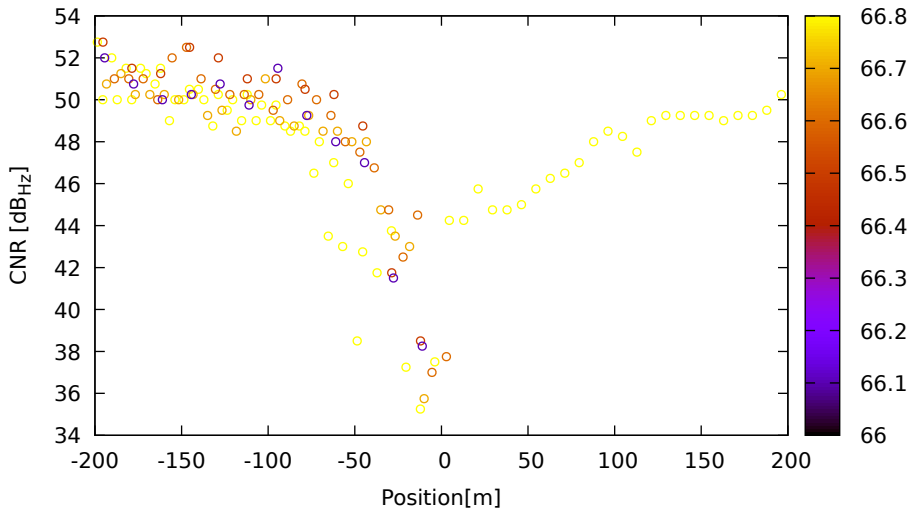
CNR vs position for E09 (E5b) on LeicaGS18 - DOY 262 jam. 1
