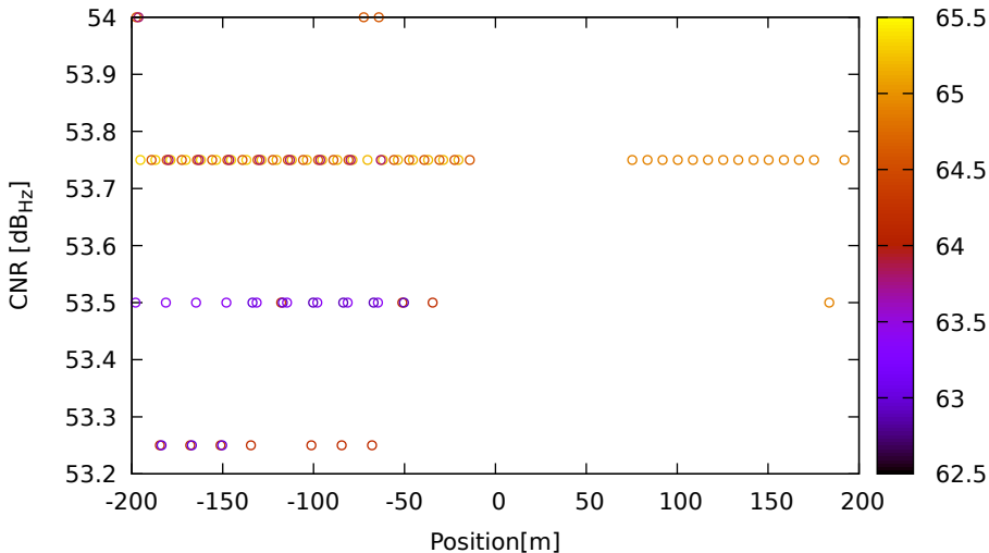
CNR vs position for E09 (E5b) on LeicaGS18 - DOY 262 jam. 2
