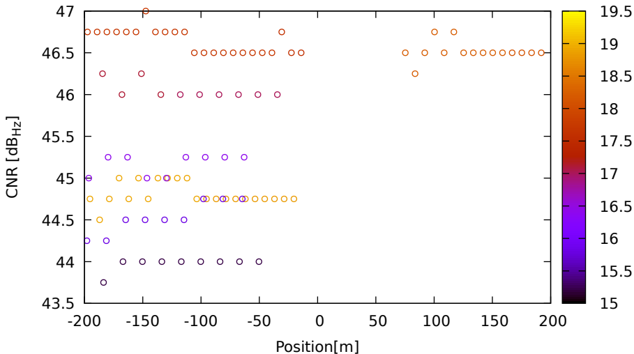
CNR vs position for E11 (E5) on LeicaGS18 - DOY 262 jam. 2
