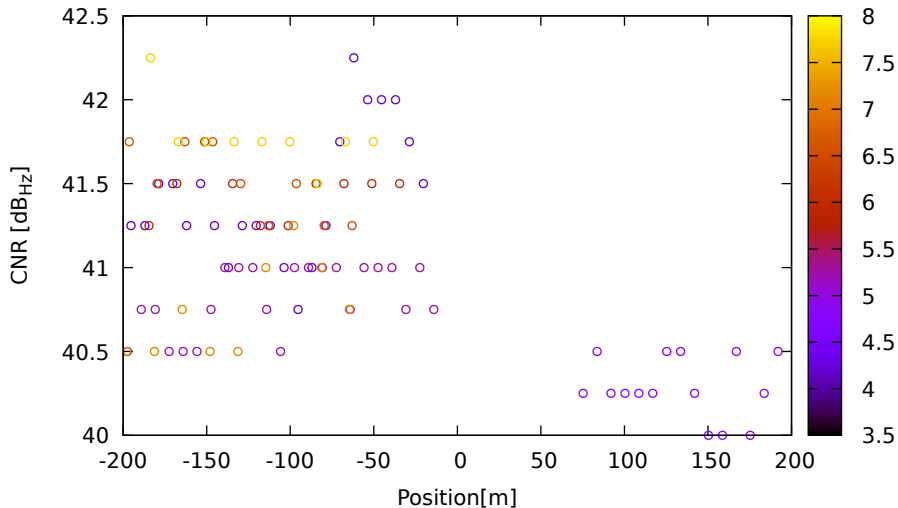
CNR vs position for E15 (E5a) on LeicaGS18 - DOY 262 jam. 2
