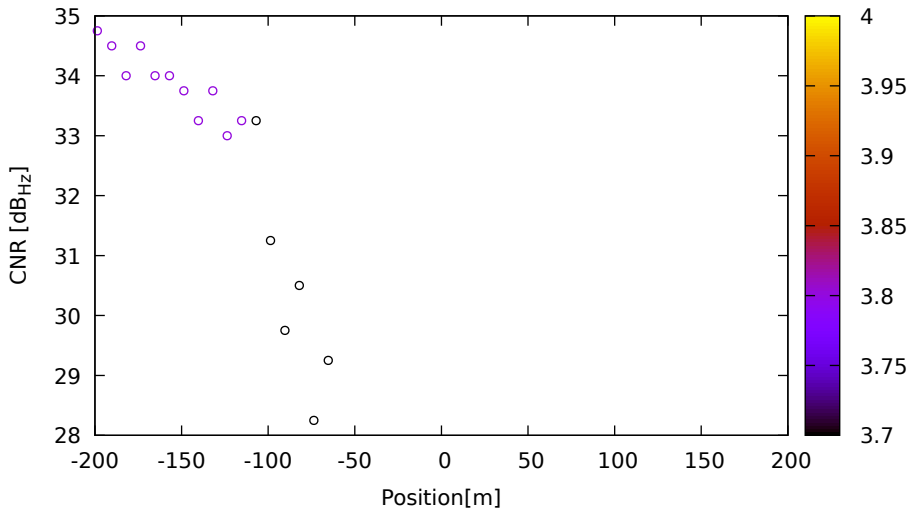
CNR vs position for E30 (E1) on LeicaGS18 - DOY 262 jam. 1
