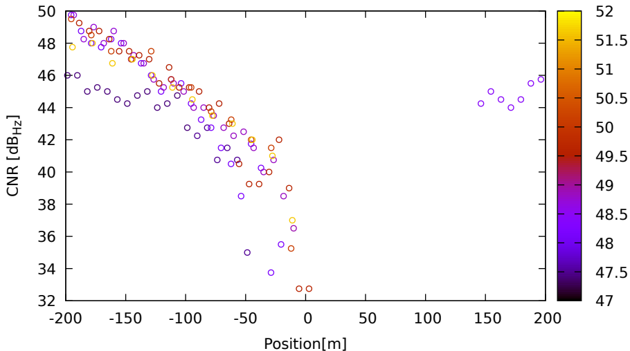
CNR vs position for E34 (E1) on LeicaGS18 - DOY 262 jam. 1
