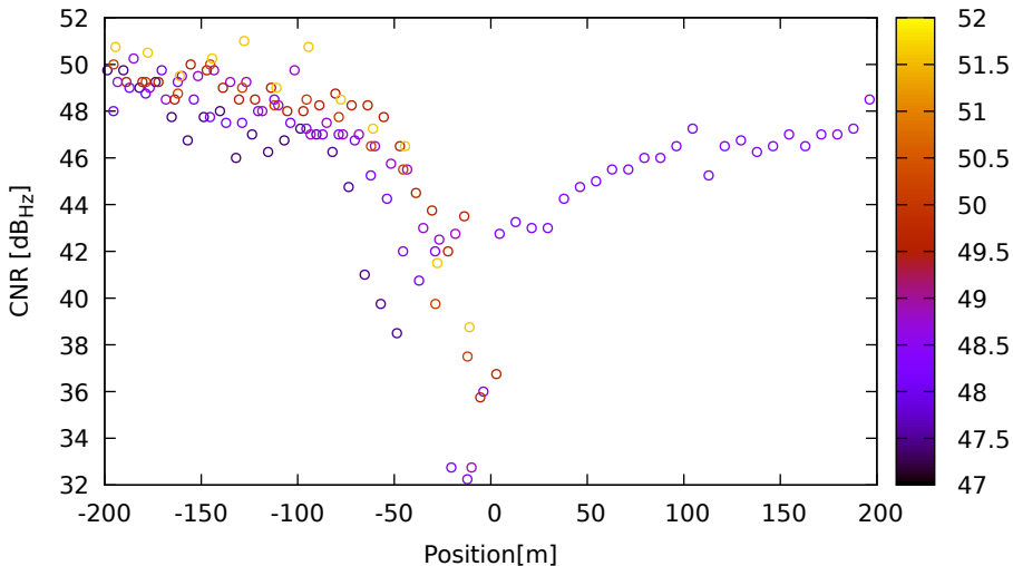
CNR vs position for E34 (E5a) on LeicaGS18 - DOY 262 jam. 1
