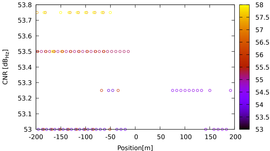
CNR vs position for E34 (E5b) on LeicaGS18 - DOY 262 jam. 2
