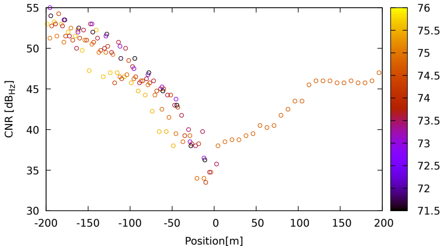
CNR vs position for E36 (E5) on LeicaGS18 - DOY 262 jam. 1
