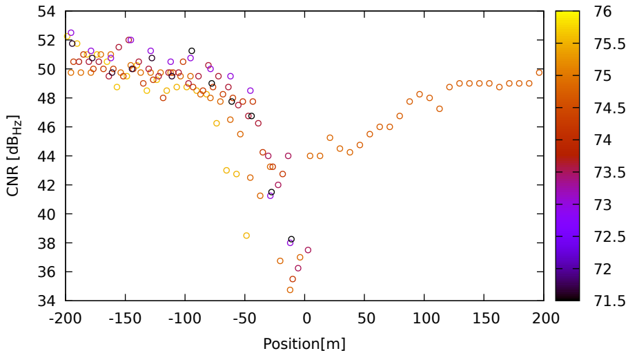
CNR vs position for E36 (E5b) on LeicaGS18 - DOY 262 jam. 1
