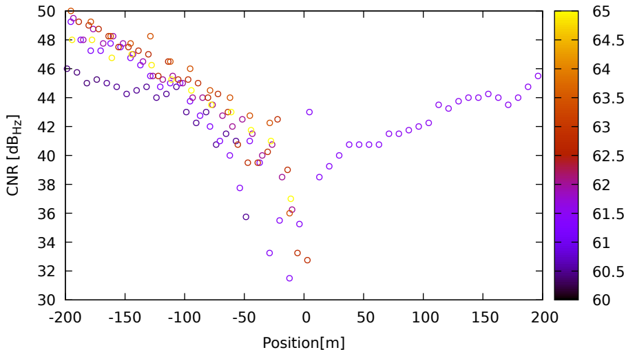
CNR vs position for G03 (L1) on LeicaGS18 - DOY 262 jam. 1
