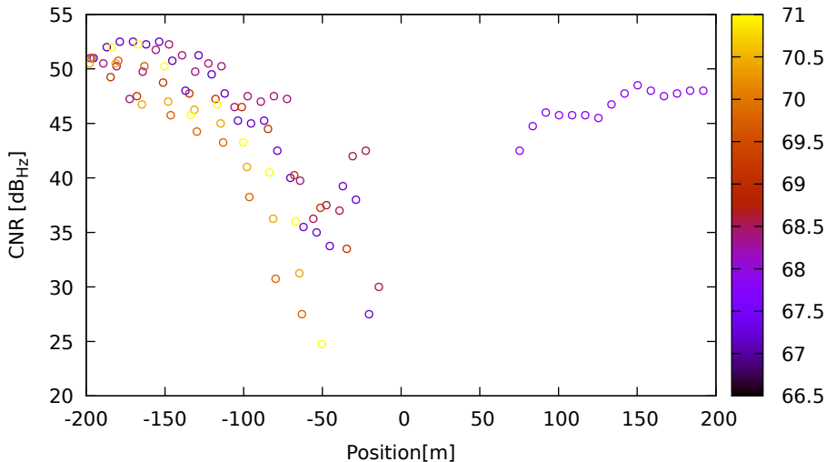
CNR vs position for G03 (L2) on LeicaGS18 - DOY 262 jam. 2
