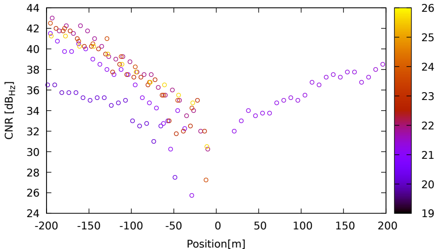
CNR vs position for G04 (L1) on LeicaGS18 - DOY 262 jam. 1
