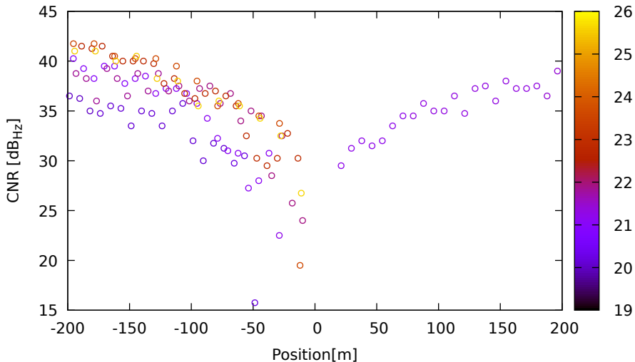
CNR vs position for G04 (L2) on LeicaGS18 - DOY 262 jam. 1
