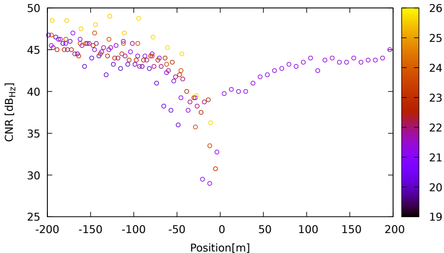
CNR vs position for G04 (L5) on LeicaGS18 - DOY 262 jam. 1
