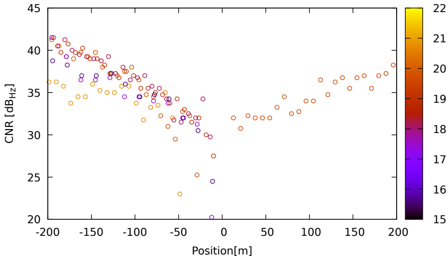
CNR vs position for G08 (L2) on LeicaGS18 - DOY 262 jam. 1
