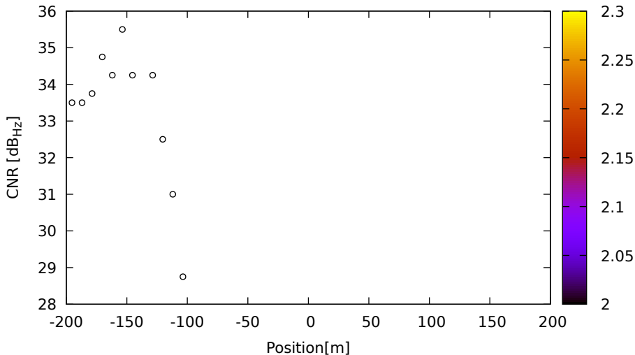
CNR vs position for G14 (L1) on LeicaGS18 - DOY 262 jam. 2
