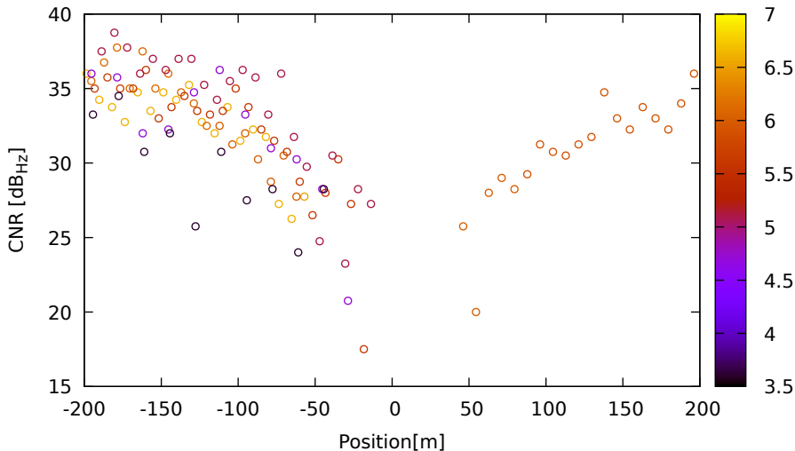
CNR vs position for G14 (L2) on LeicaGS18 - DOY 262 jam. 1
