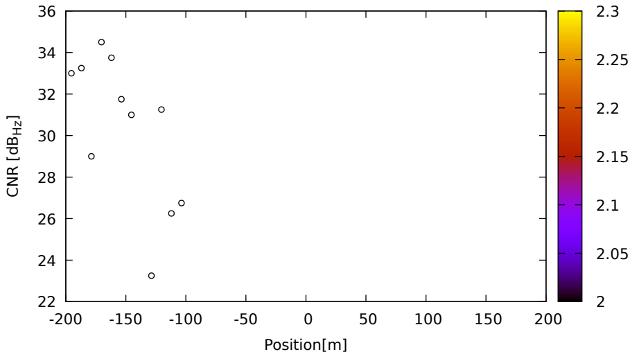
CNR vs position for G14 (L2) on LeicaGS18 - DOY 262 jam. 2
