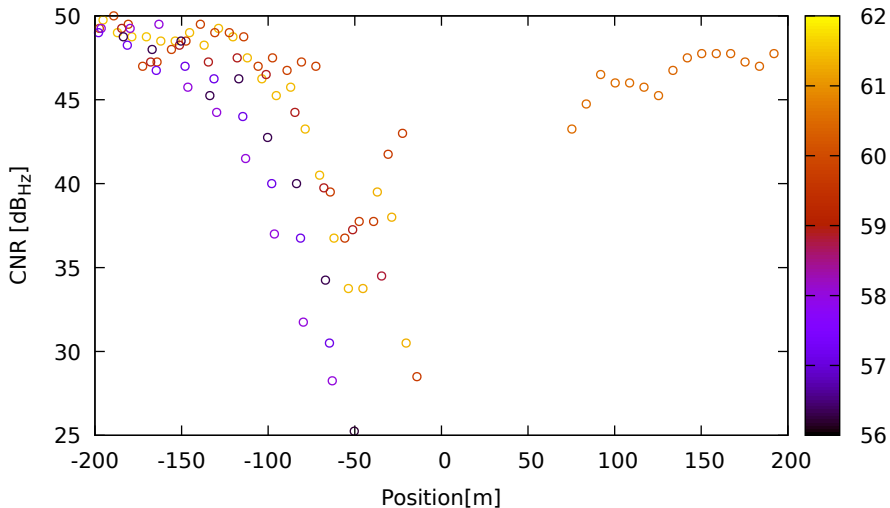
CNR vs position for G21 (L2) on LeicaGS18 - DOY 262 jam. 2
