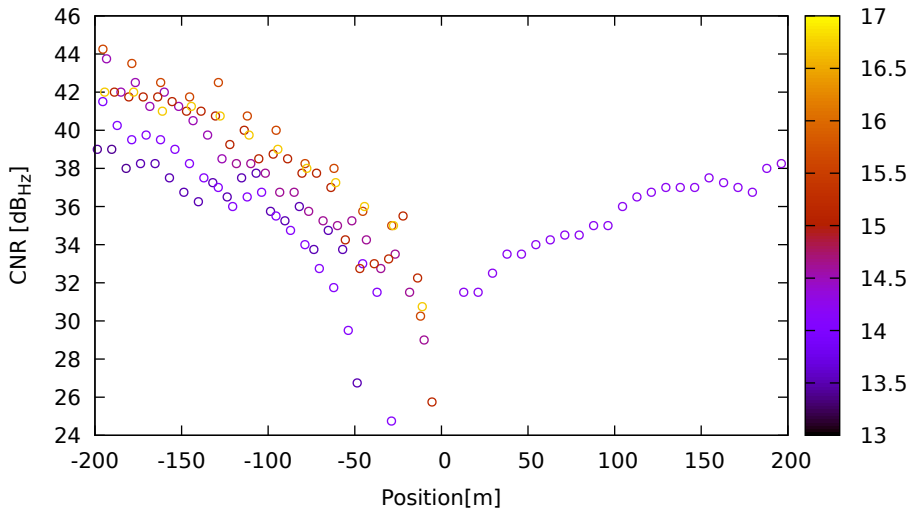
CNR vs position for G31 (L1) on LeicaGS18 - DOY 262 jam. 1
