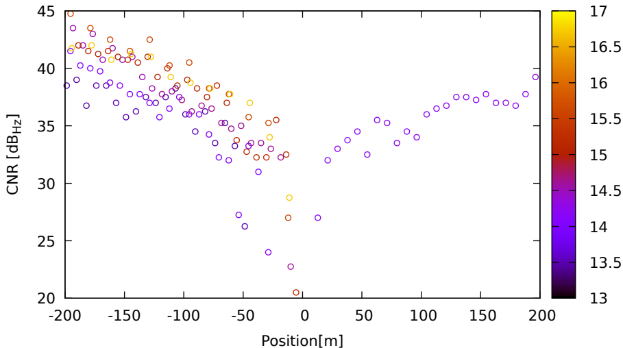
CNR vs position for G31 (L2) on LeicaGS18 - DOY 262 jam. 1
