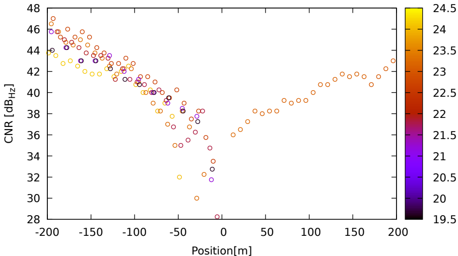
CNR vs position for G32 (L1) on LeicaGS18 - DOY 262 jam. 1
