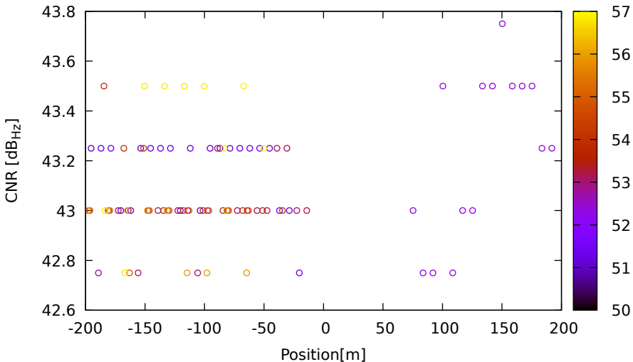
CNR vs position for R01 (G2) on LeicaGS18 - DOY 262 jam. 2
