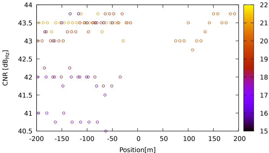
CNR vs position for R07 (G2) on LeicaGS18 - DOY 262 jam. 2
