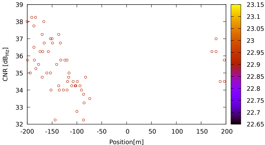
CNR vs position for C05 (B1) on LeicaGS18 - DOY 262 jam. 1
