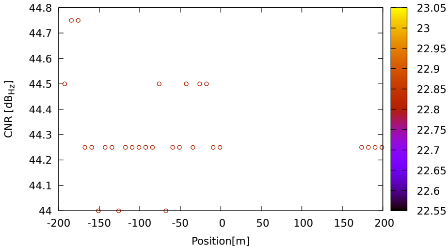
CNR vs position for C05 (B2) on LeicaGS18 - DOY 262 jam. 3
