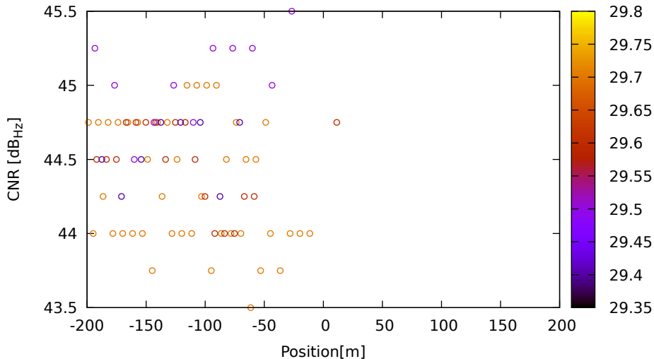
CNR vs position for C06 (B2) on LeicaGS18 - DOY 262 jam. 2
