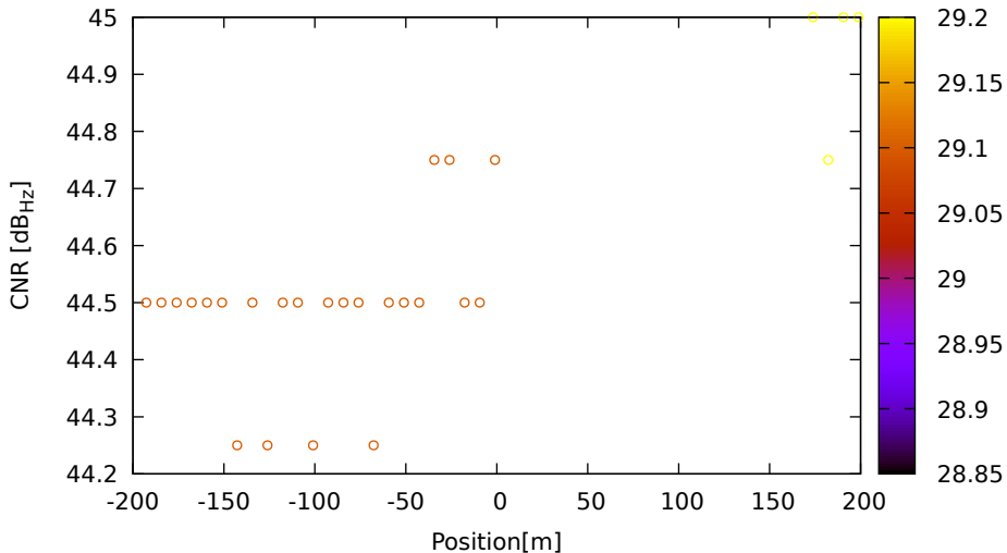
CNR vs position for C06 (B2) on LeicaGS18 - DOY 262 jam. 3
