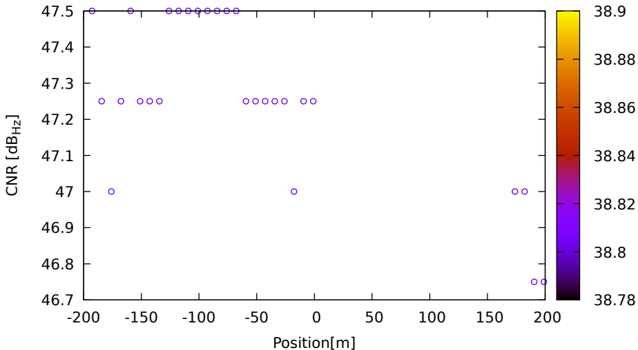
CNR vs position for C09 (B2) on LeicaGS18 - DOY 262 jam. 3
