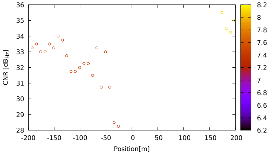
CNR vs position for C11 (B1) on LeicaGS18 - DOY 262 jam. 3
