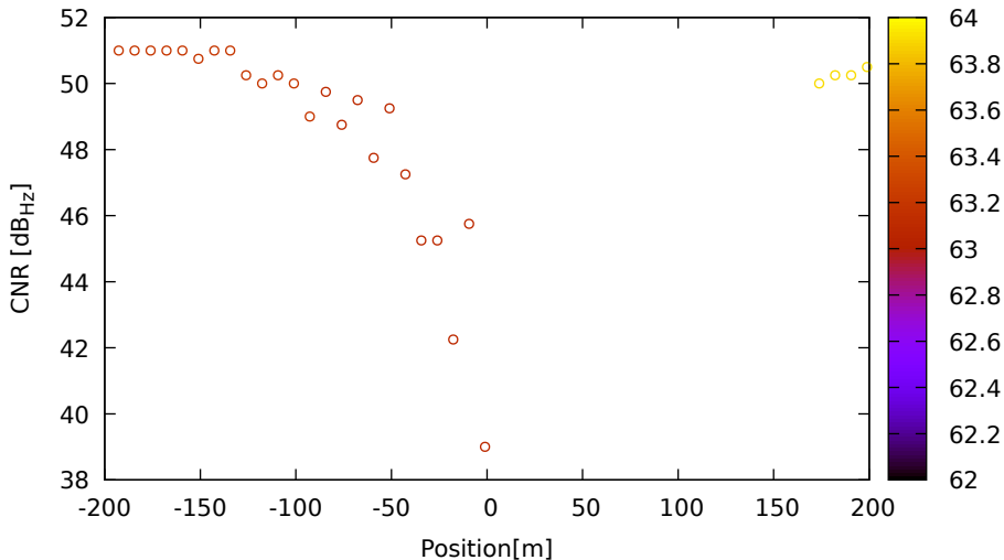
CNR vs position for C14 (B1) on LeicaGS18 - DOY 262 jam. 3
