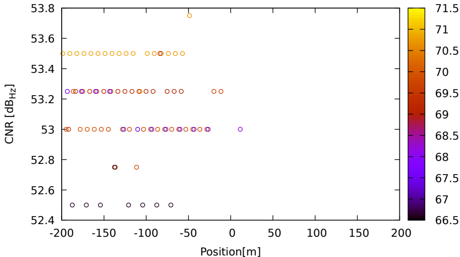
CNR vs position for C14 (B2) on LeicaGS18 - DOY 262 jam. 2
