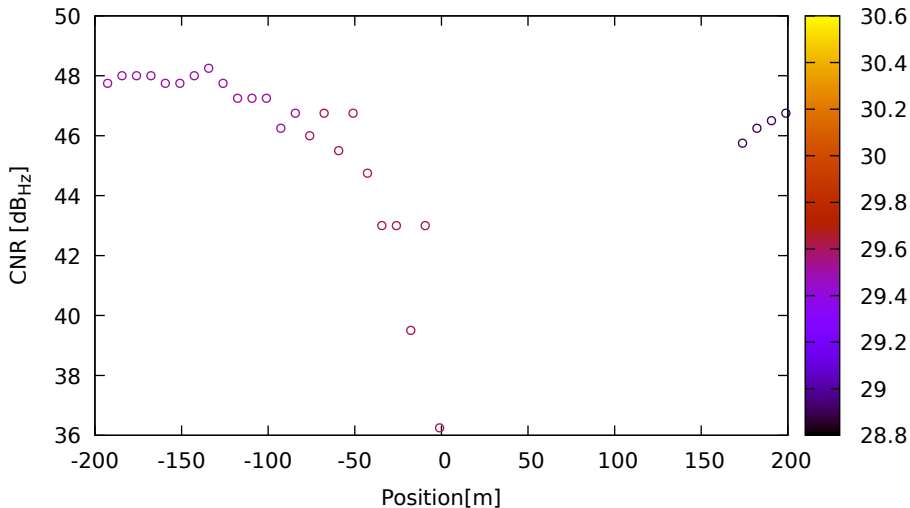
CNR vs position for C27 (B1) on LeicaGS18 - DOY 262 jam. 3
