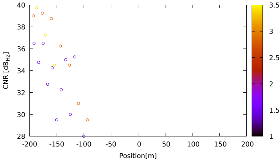
CNR vs position for E03 (E1) on LeicaGS18 - DOY 262 jam. 2
