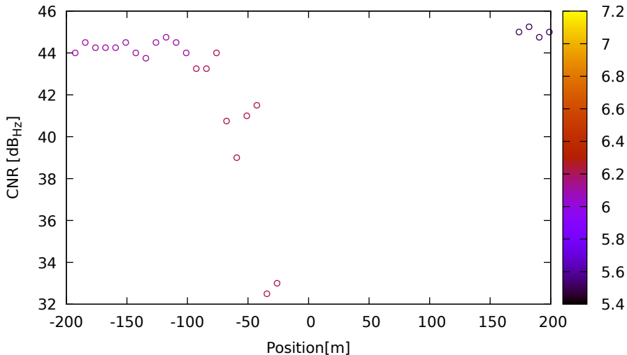
CNR vs position for E03 (E1) on LeicaGS18 - DOY 262 jam. 3
