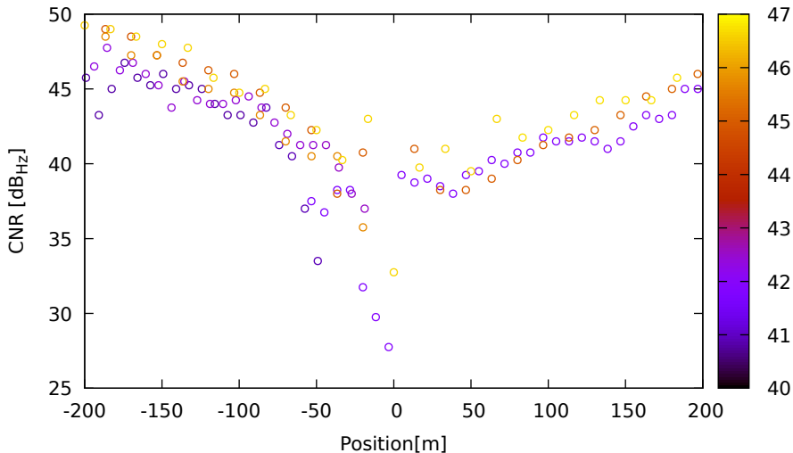
CNR vs position for E05 (E1) on LeicaGS18 - DOY 262 jam. 1
