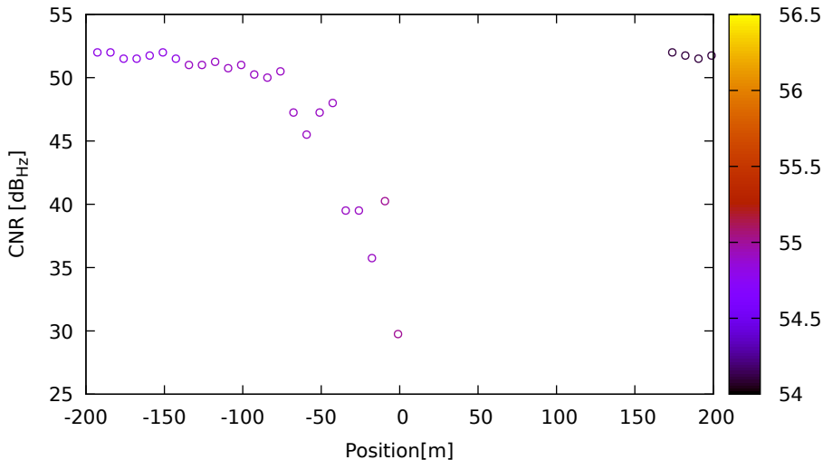
CNR vs position for E05 (E1) on LeicaGS18 - DOY 262 jam. 3
