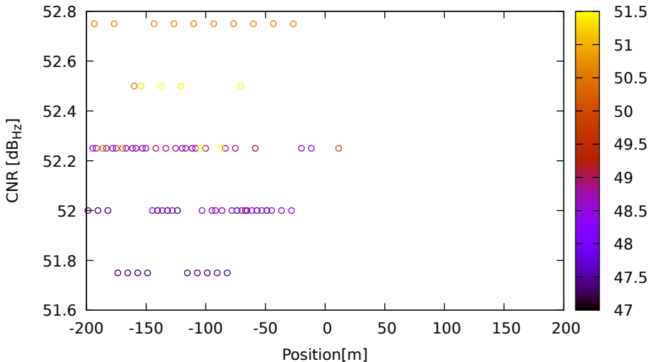
CNR vs position for E05 (E5b) on LeicaGS18 - DOY 262 jam. 2
