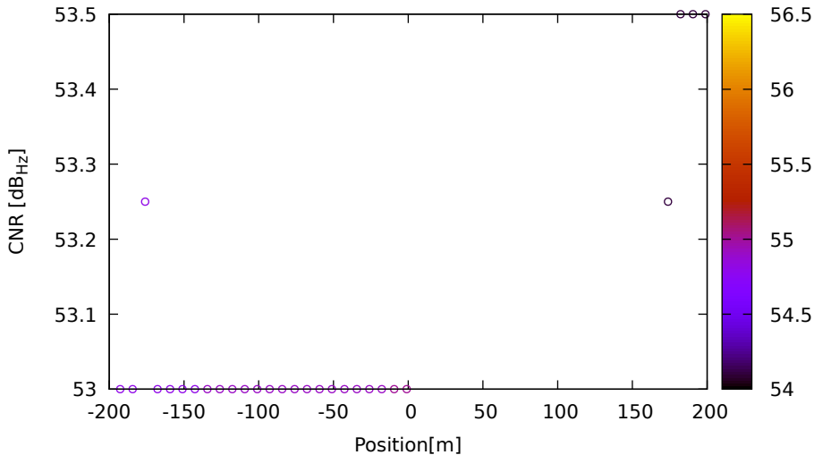
CNR vs position for E05 (E5b) on LeicaGS18 - DOY 262 jam. 3
